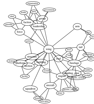
Figure 2: Local graph of the word wing
